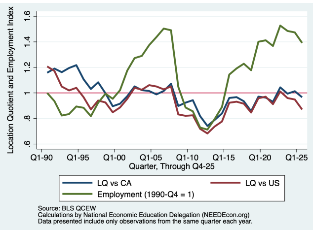
Figure 2 - 8: Construction
