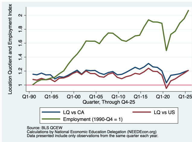
Figure 2 - 3: Educ. Services
