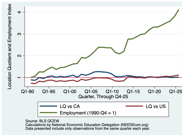
Figure 2 - 3: Educ. Services
