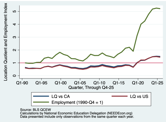
Figure 2 - 6: Trans. & Ware.
