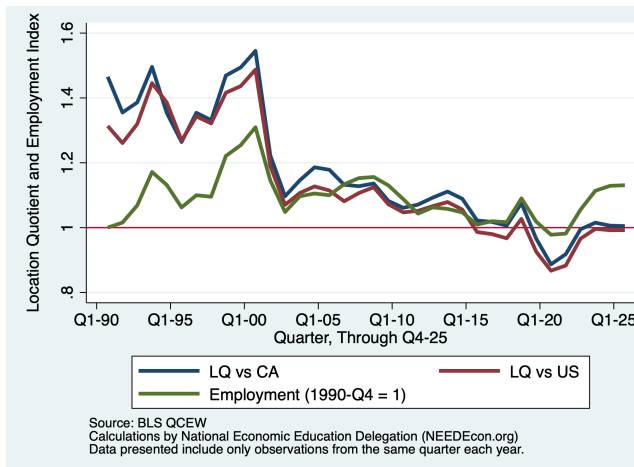
Figure 2 - 7: Public Admin
